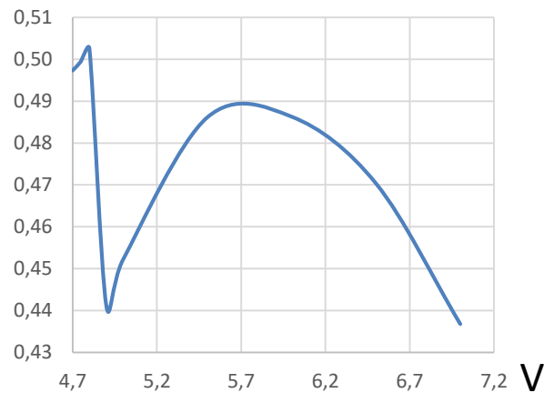
e Efficiency @350 mA load
