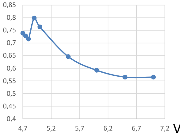
A Consumption @350 mA load
